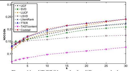
Figure 11. NDCG@k results for different methods.
